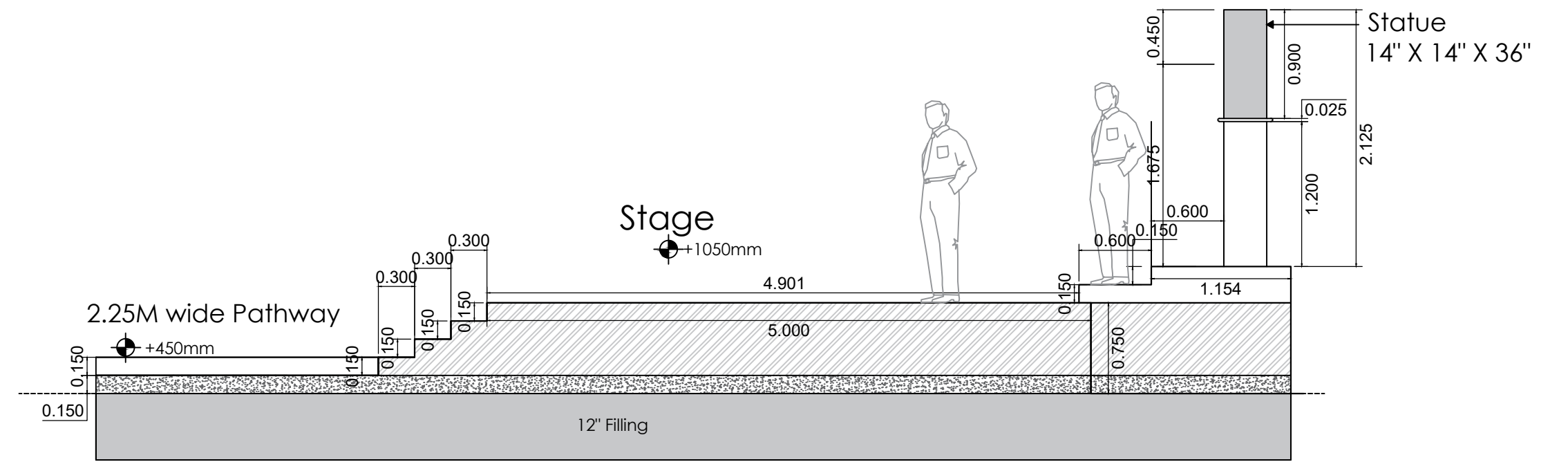
Section D-D'
